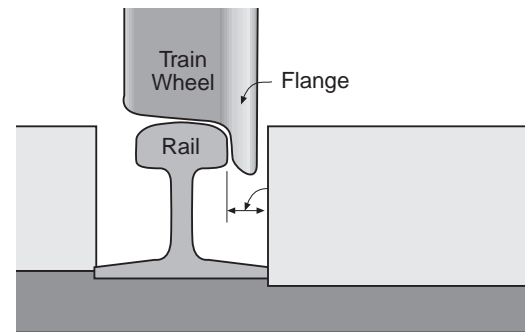
Fig. 2-40: Federal regulations require the gauge flangeway to be a minimum of 2.5in. wide to allow for the train wheel flange.
