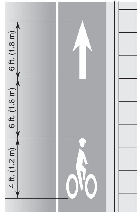
Figure 3-28: The standard marking for a bicycle lane is the bicyclist symbol accompanied by an arrow.
