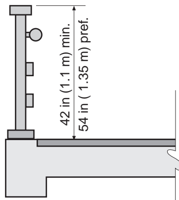
Figure 4-120: Railings should be high enough to prevent pitchover.
