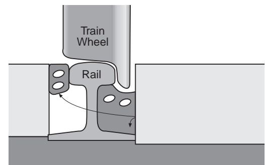
Fig. 2-41: Fillers can completely eliminate the field flangeway gap but must allow for the train wheel in the gauge flangeway.
