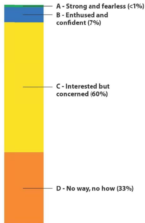
Figure 3-1 Bicyclist Classifications
